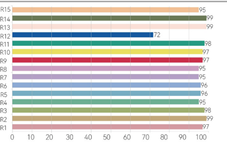
RGBTD 5-in-1 DAYLIGHT COLOR RENDERING INDEX CCT 6479K Ra=96.2
